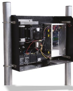
Figure 15-11 HySecurity Slidesmart HD
