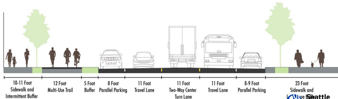
Missing Link Proposed Condition NW Market St Cross Section 100 Foot Right-of-Way
