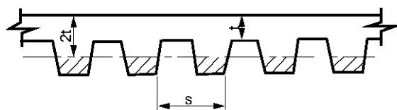
FIGURE 722.2.2.1.2 DETERMINATION OF SLAB THICKNESS FOR SLOPING SOFFITS
