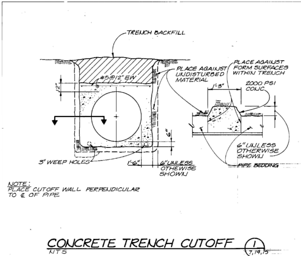
Figure 5-22 Trench Cutoff Example
