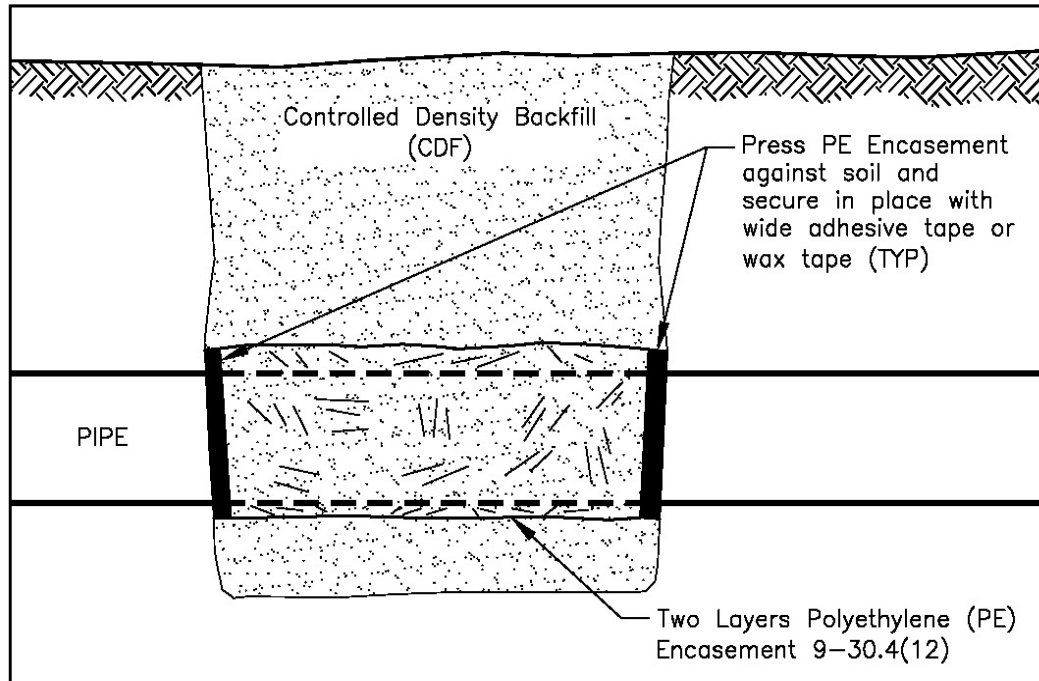
Figure 5-4 Controlled Density Fill
