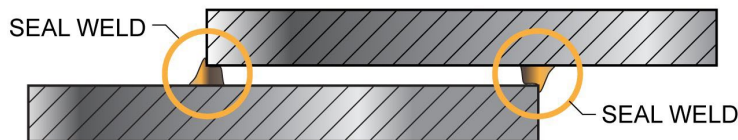
Figure 5-23 Seal Welds
