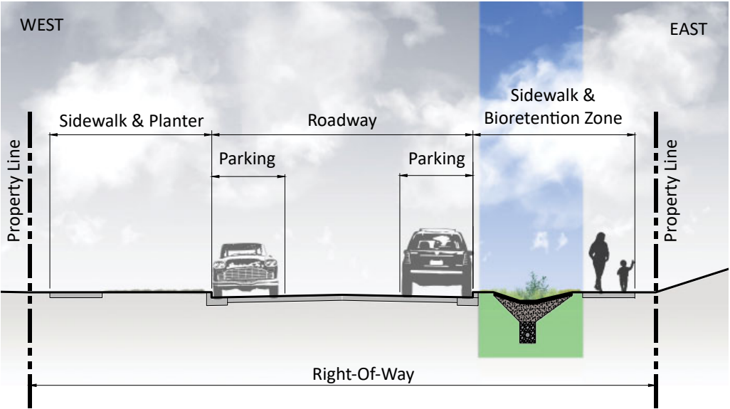
17th Ave SW — Proposed
