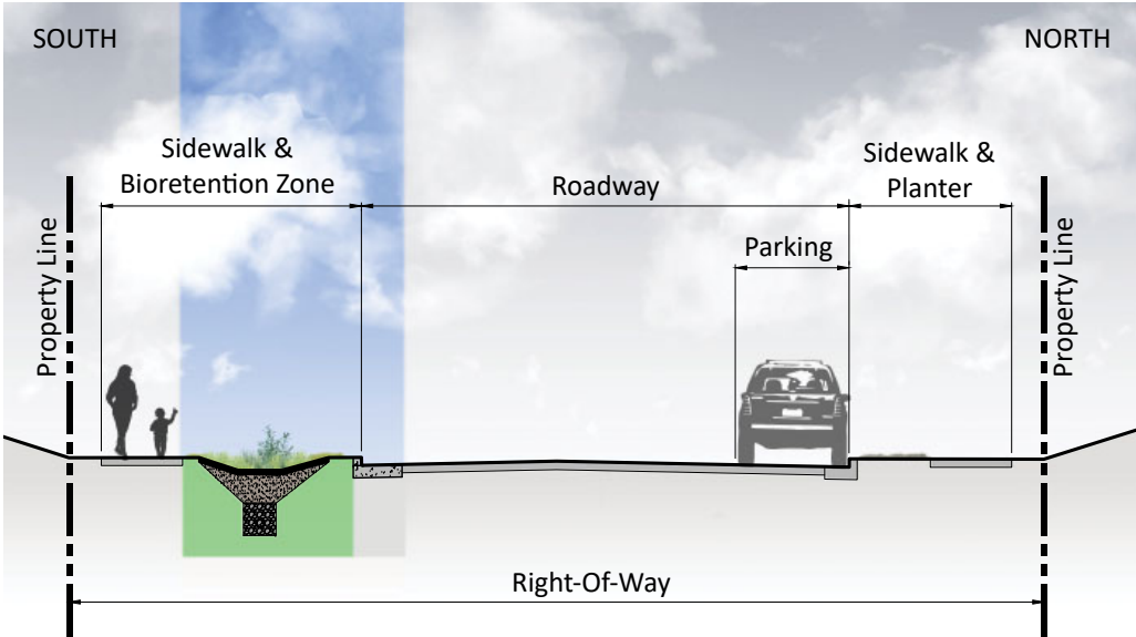
SW Holden St — Proposed
