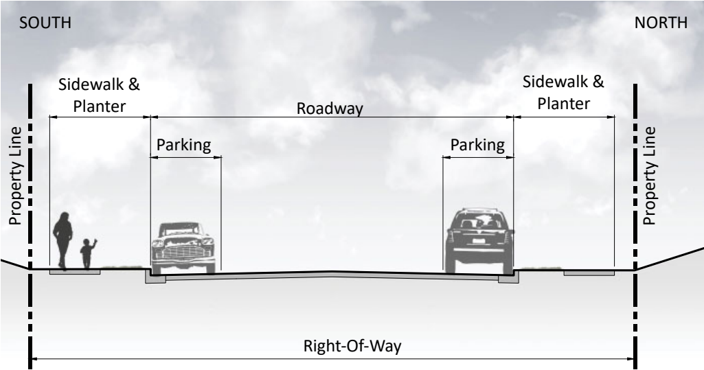
SW Holden St Curb Bump-Out @ 17th Ave SW — Existing
