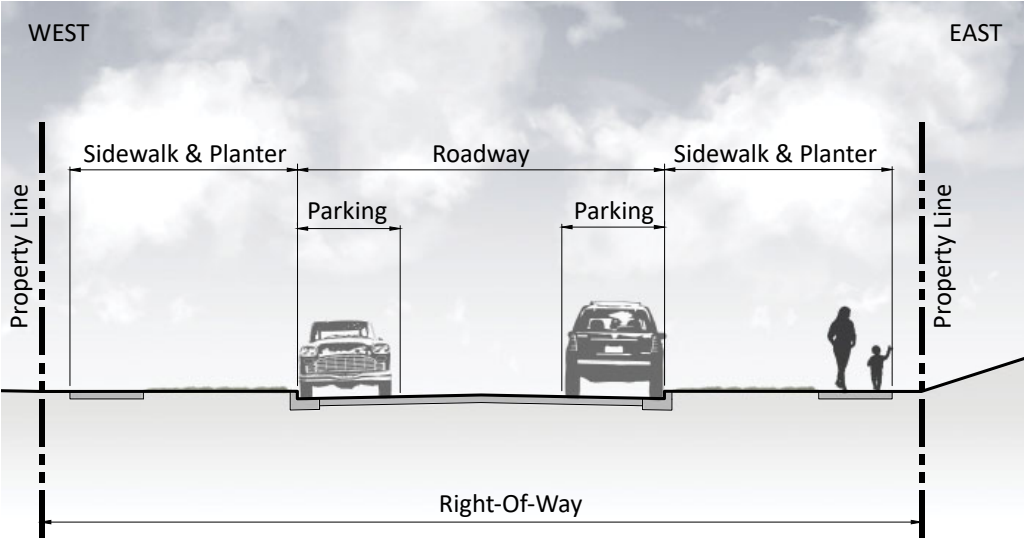
17th Ave SW — Existing
