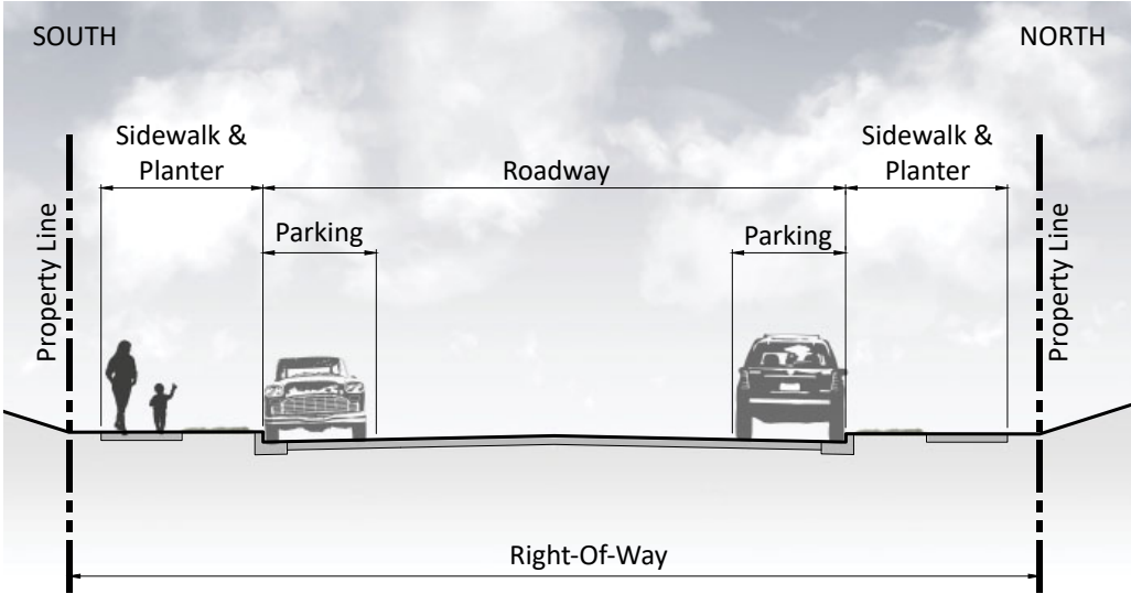
SW Holden St — Existing
