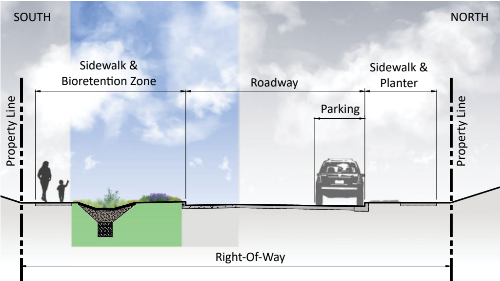
SW Holden St Curb Bump-Out @ 17th Ave SW — Proposed
