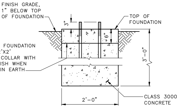
IN EARTH
