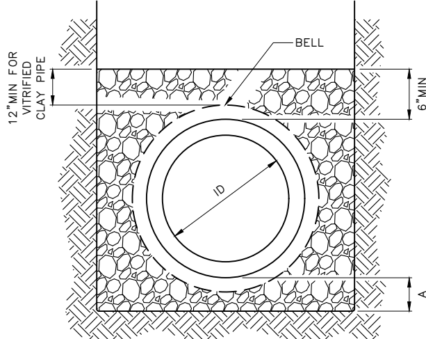
CLASS B BEDDING
