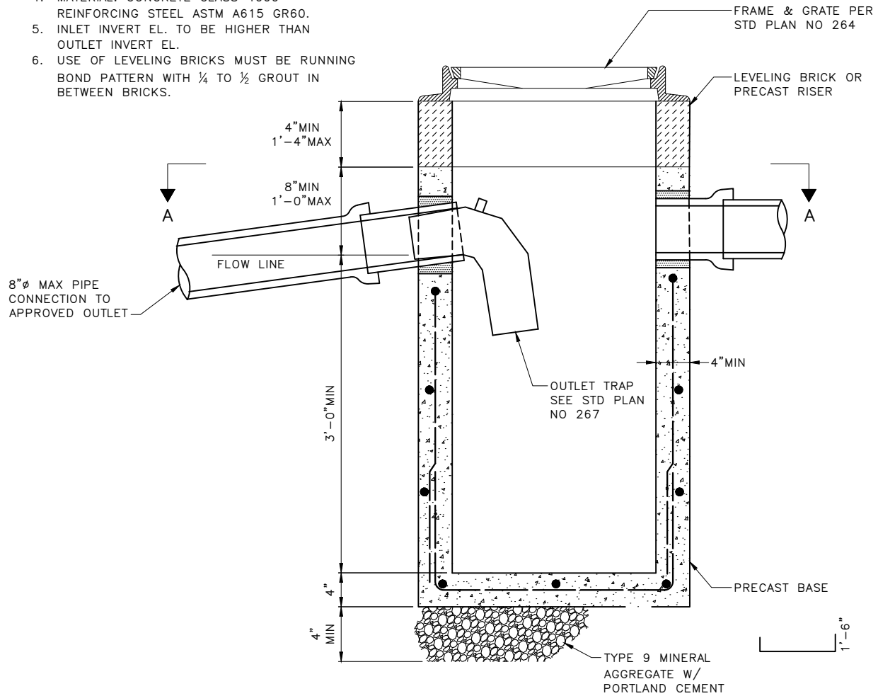
SECTION B-B
