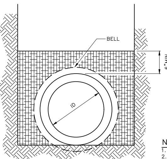
CLASS D BEDDING
