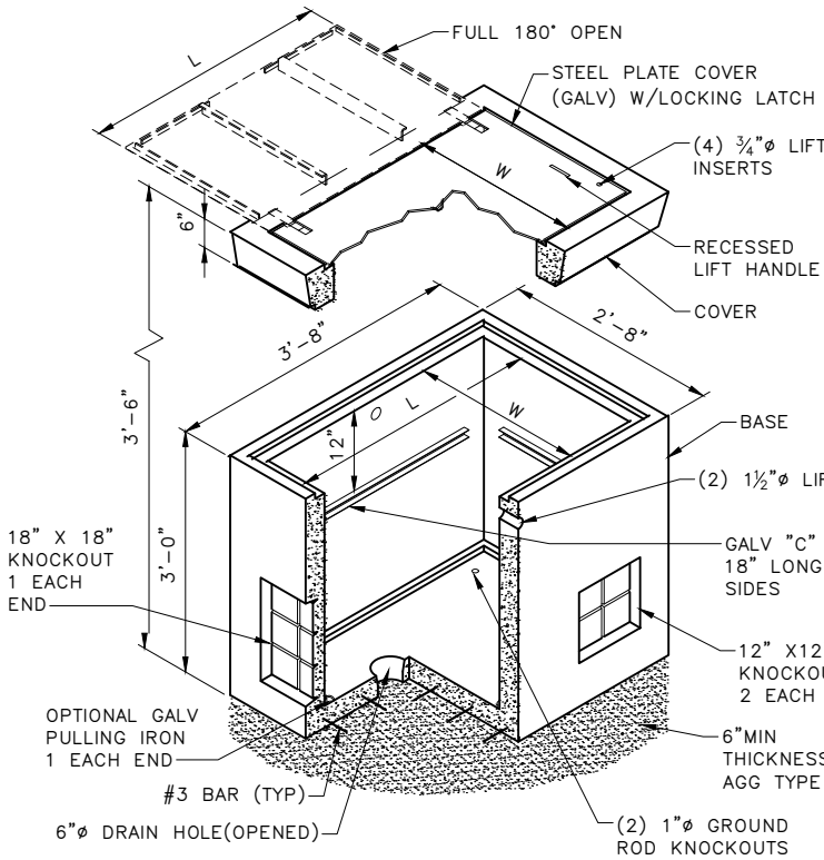
TYPE 5 HANDHOLE
