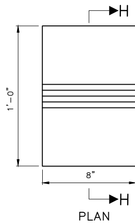
RADIAL CURB
