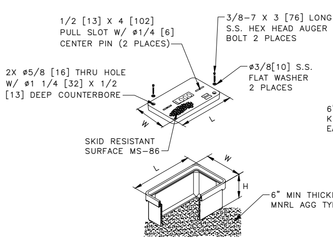
TYPE 1 & 2 HANDHOLE
