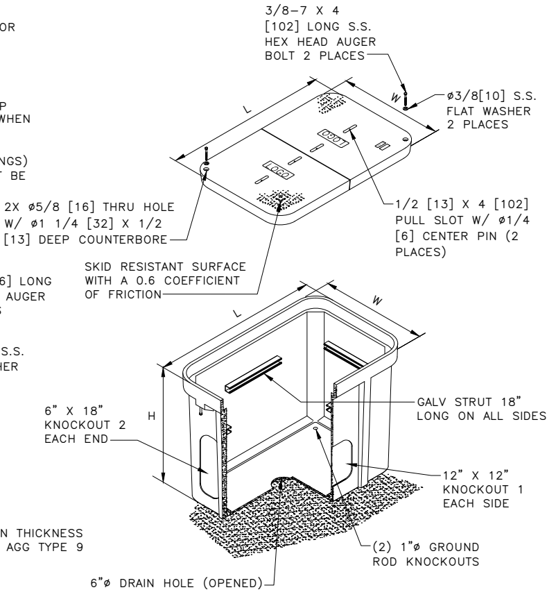
TYPE 5 HANDHOLE
