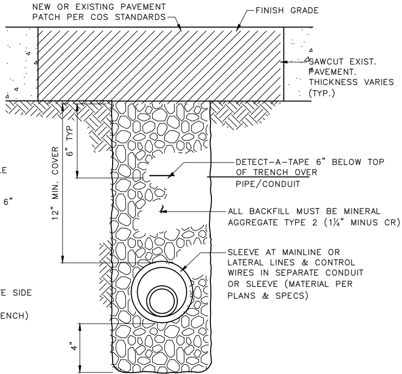
IRRIGATION SLEEVE TRENCHING UNDER PATHWAY OR SIDEWALK
