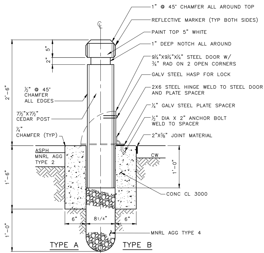
REMOVABLE BOLLARDS
