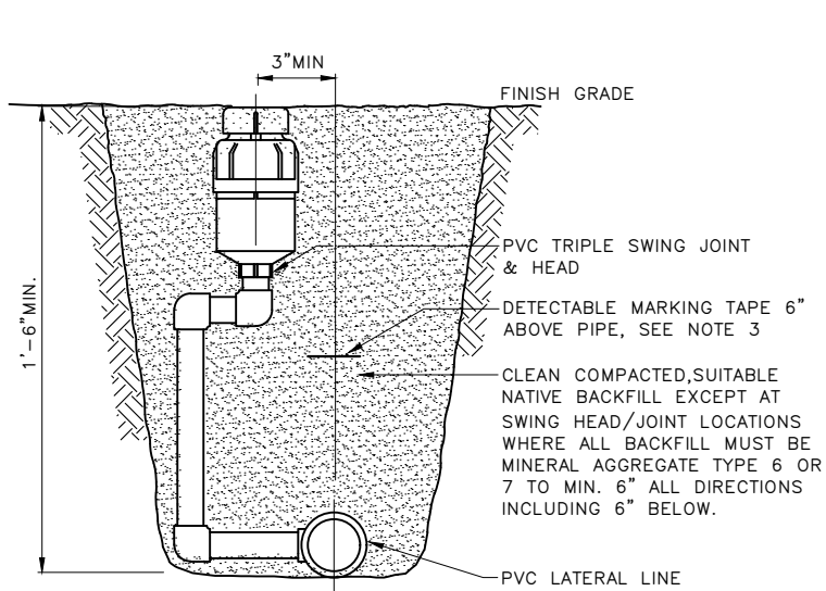
LATERAL LINE
