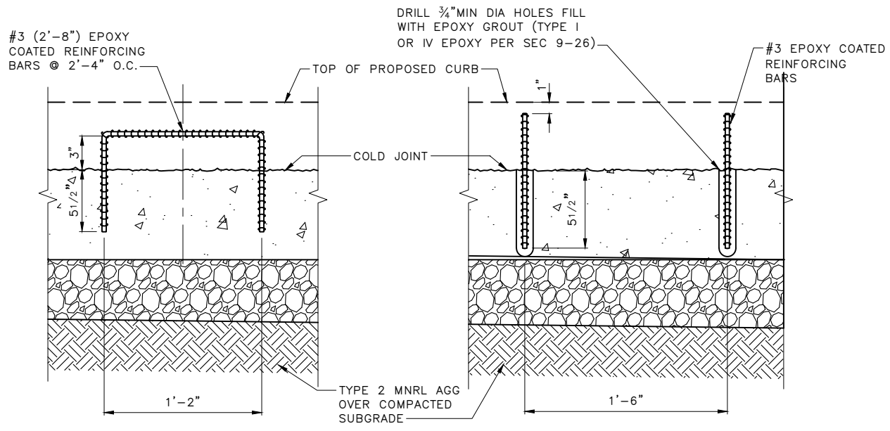
CURB DOWEL ON NEW PAVEMENT
