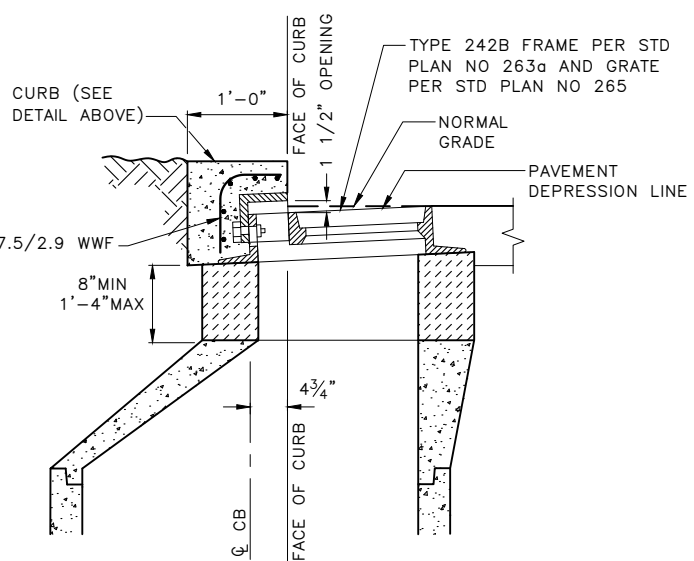
TYPE 242B CB (TYPE 250B INLET SIMILAR)
