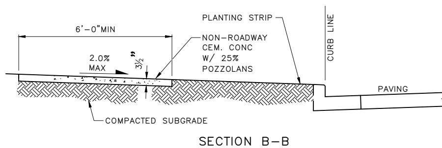
TYPICAL SIDEWALK & CURB RAMP DETAIL
