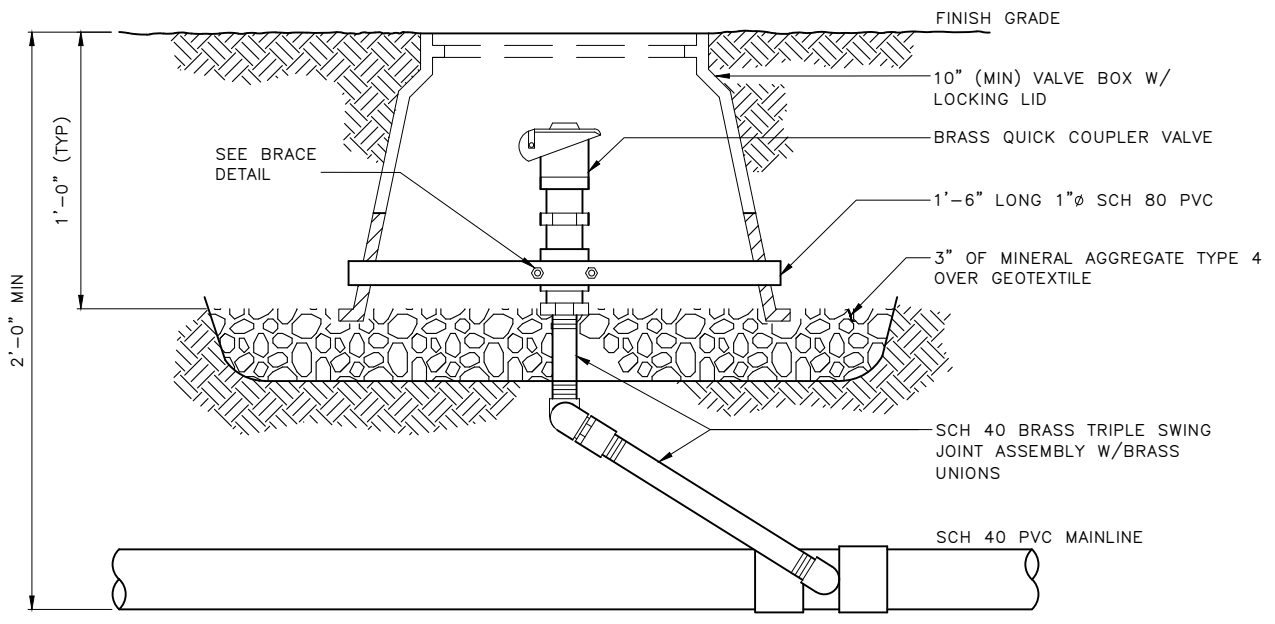
ELEVATION VIEW
