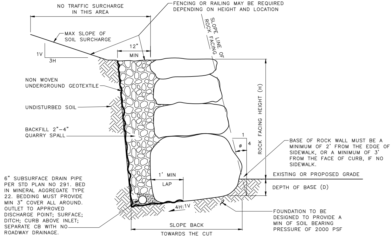
SECTION
