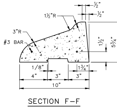
8" STRAIGHT BLOCK CURB (SINGLE SLOPED)
