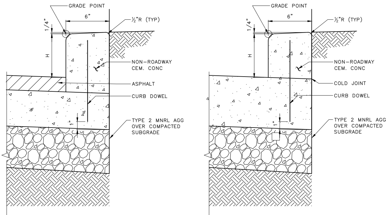
410C CURB
