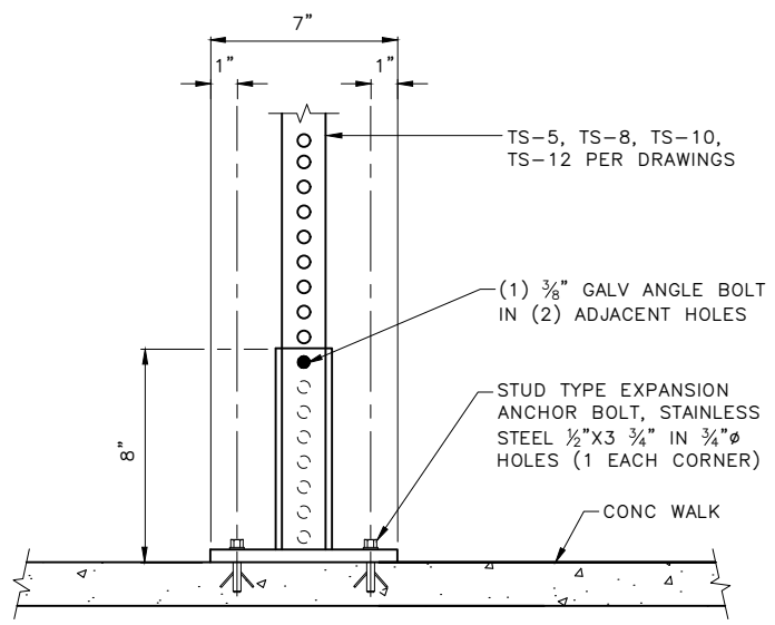
SURFACE MOUNT
