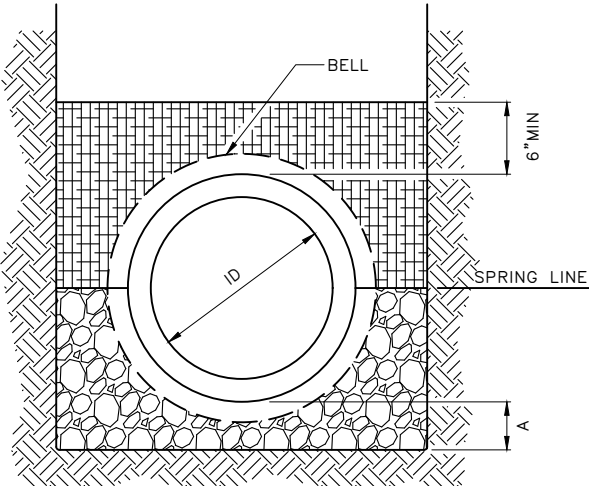
CLASS C BEDDING
