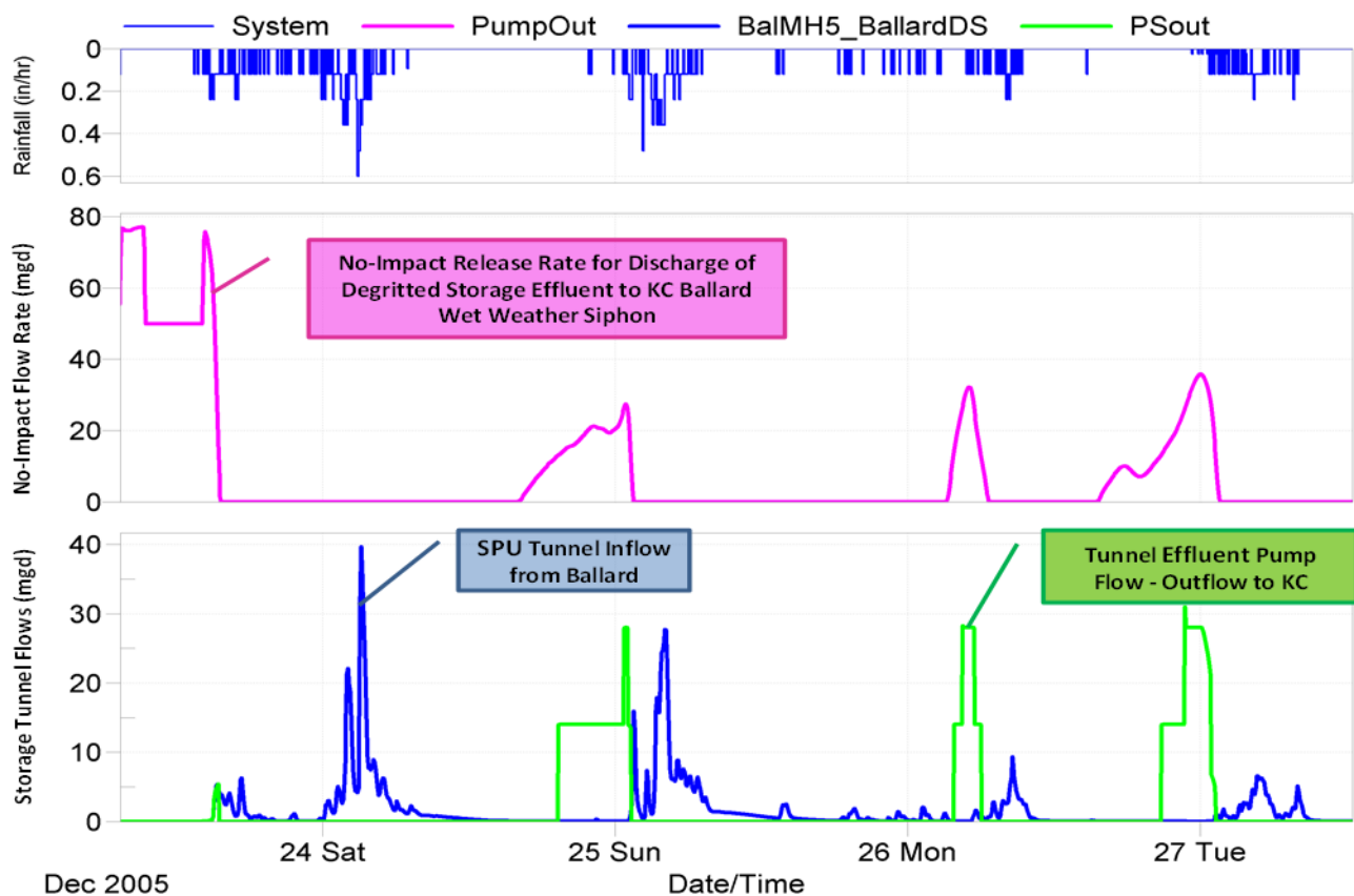
Figure 5-29. Example of Shared West Ship Canal Tunnel Storage Operation During CSO Event
