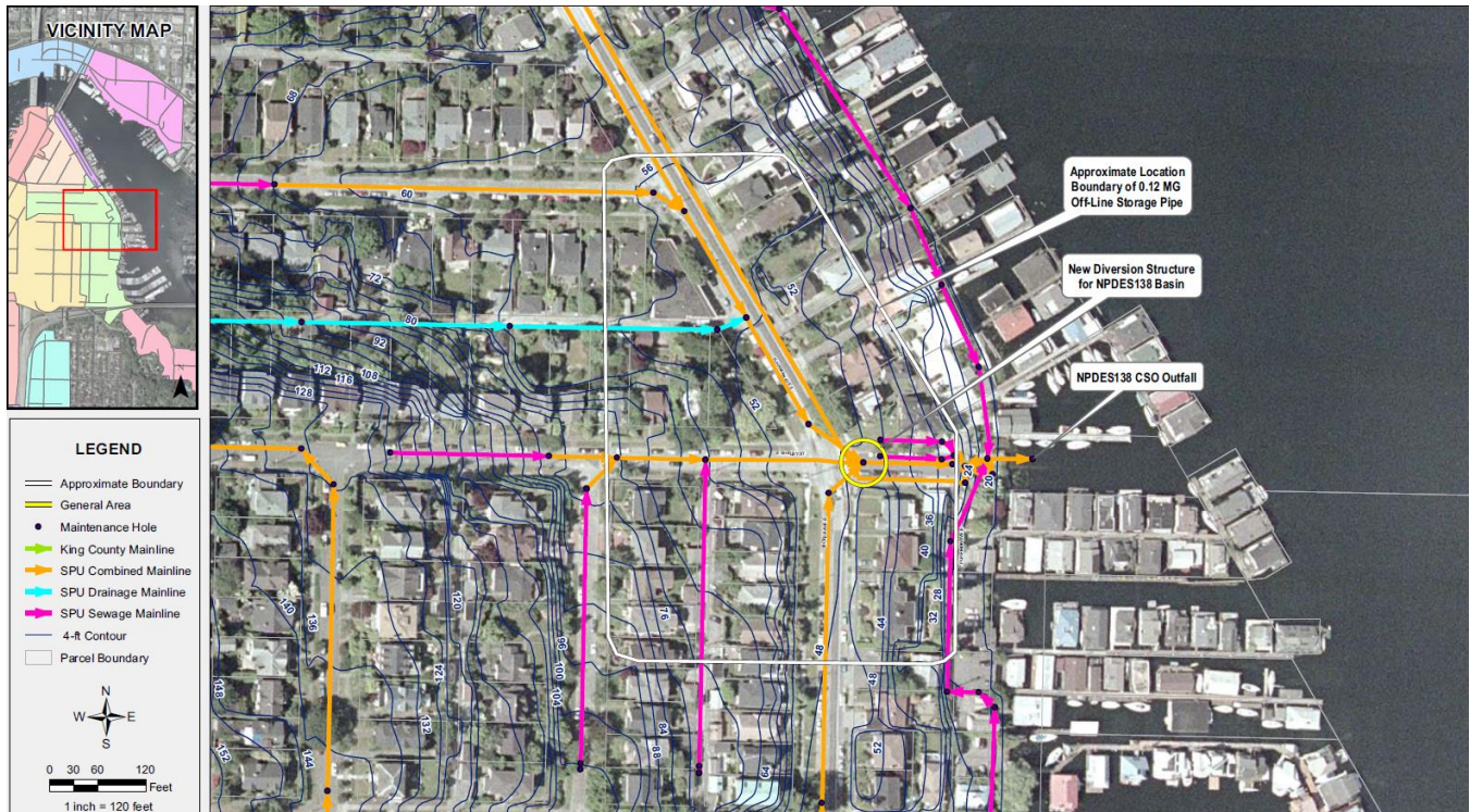
Figure 5-25. Portage Bay/Lake Union CSO Outfall 138 Recommended Control Measure
