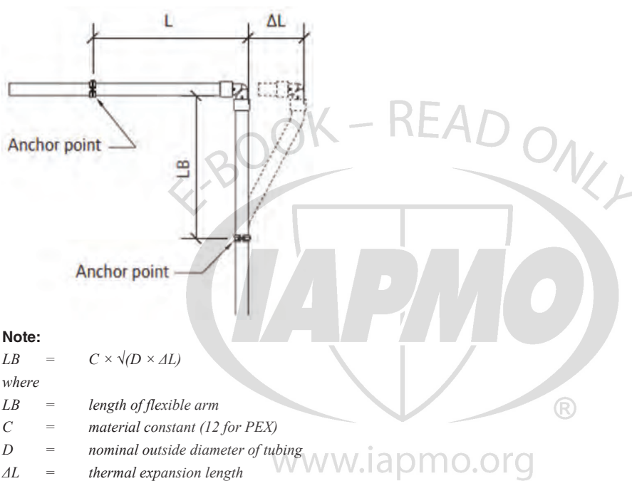
FIGURE 1 EXPANSION ARMS (See Sections 6.4.1 and 7.3)
