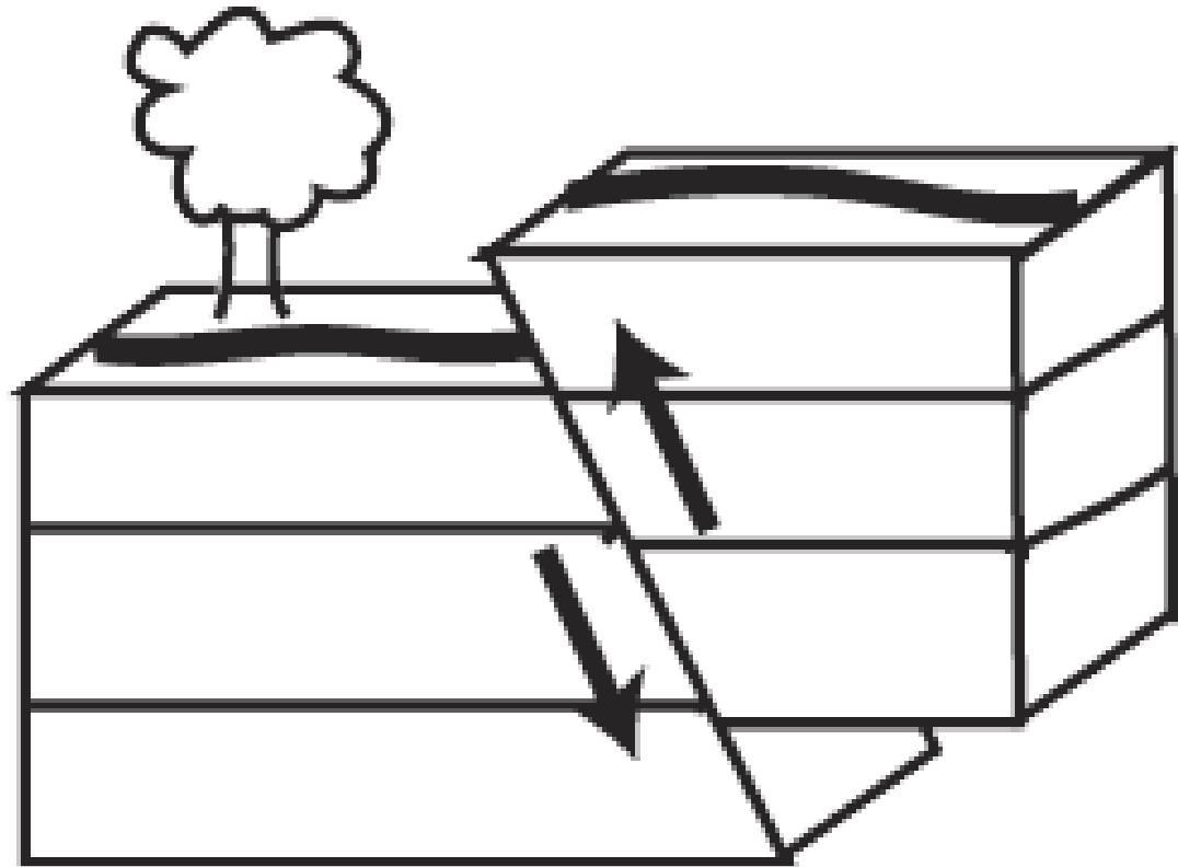
Thrust Fault
