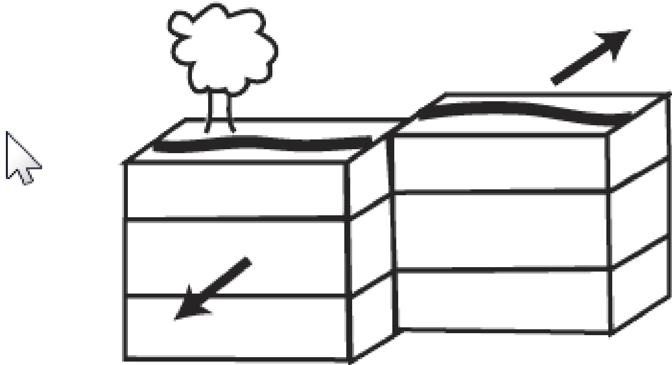
Strike-slip Fault
