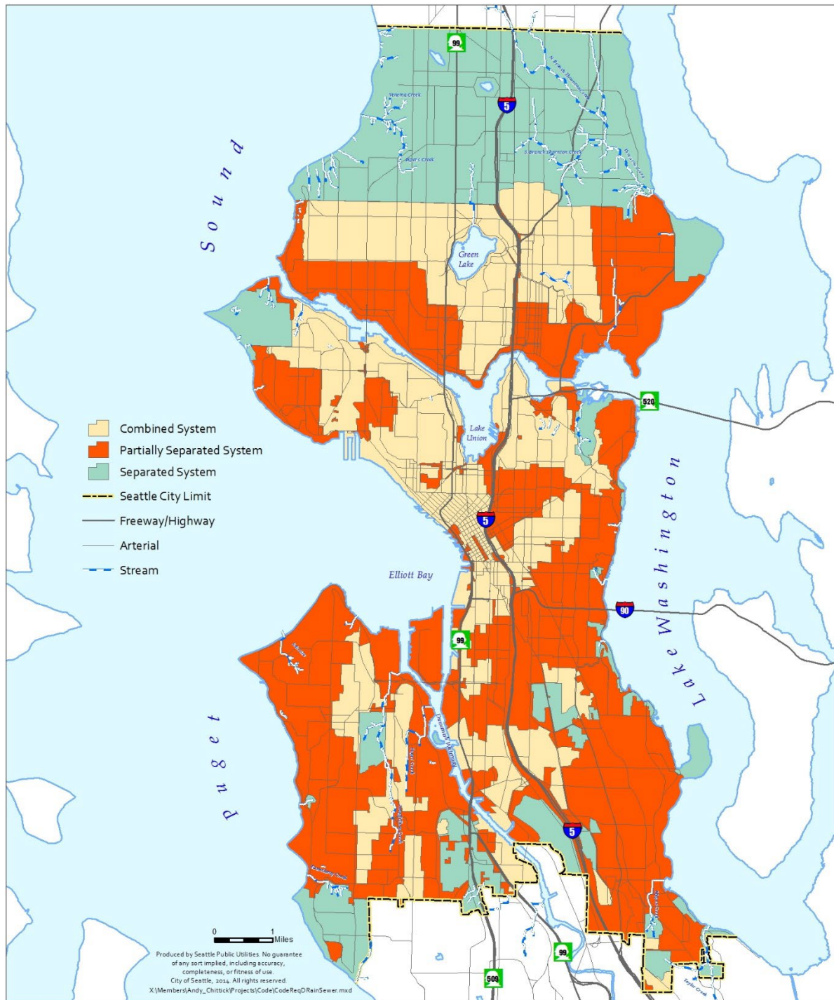
Figure 2.78. Public Combined Sewer Basins.
