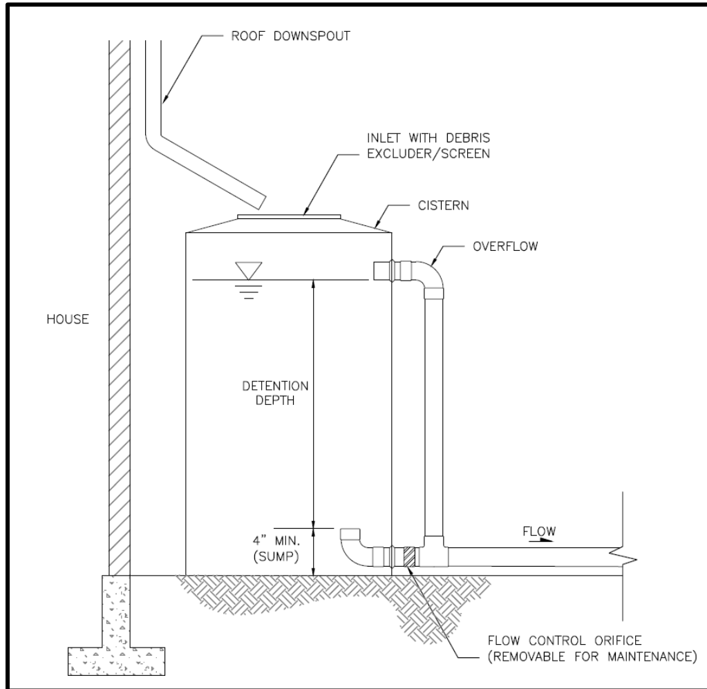
Figure 5.3330. Detention Cistern.
