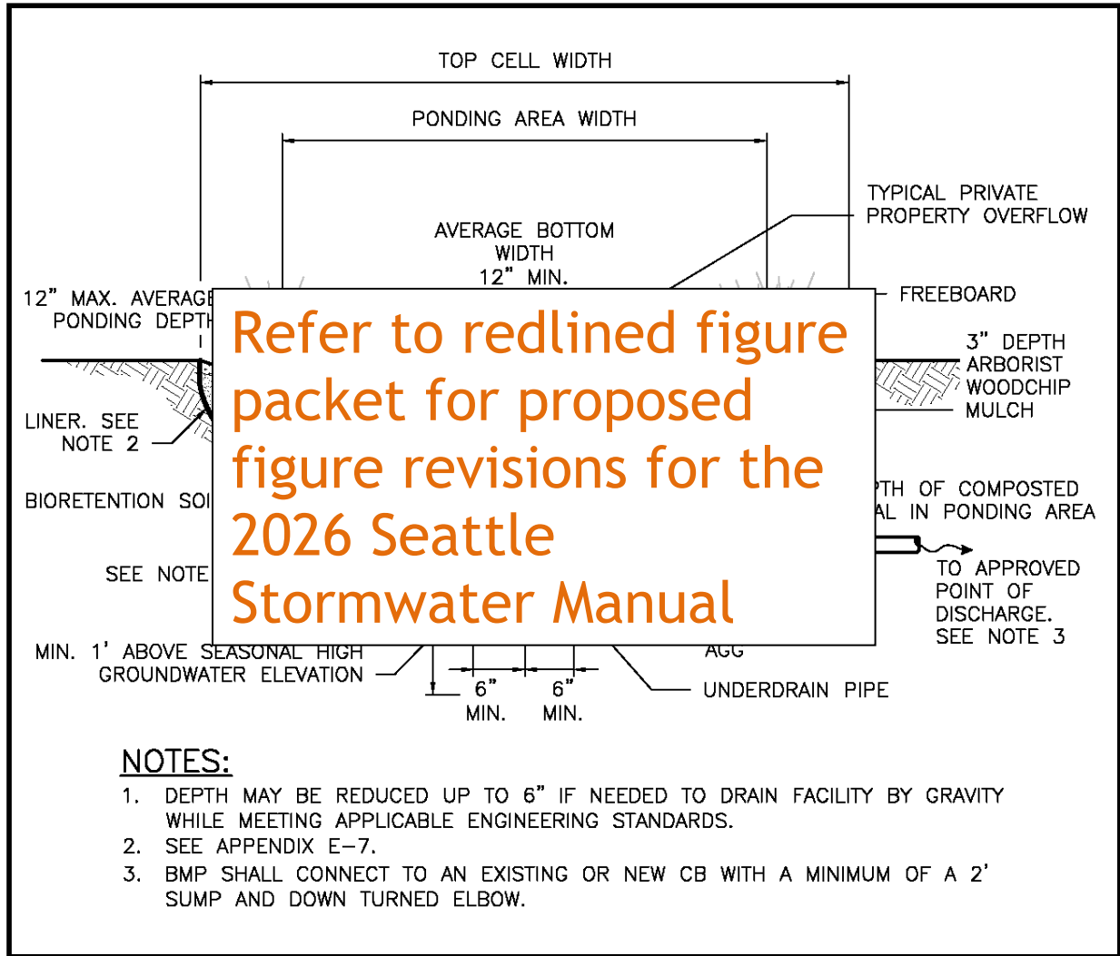
Figure 5.3434. Non-infiltrating Bioretention Facility with Sloped Sides.
