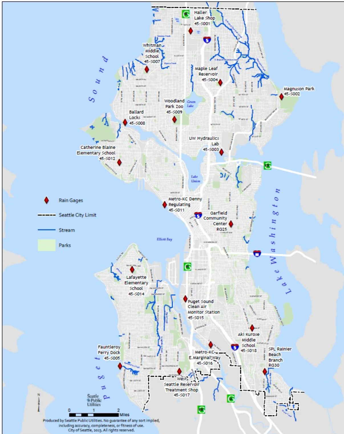
Figure F.1. Active City Rain Gauge Network Stations.
