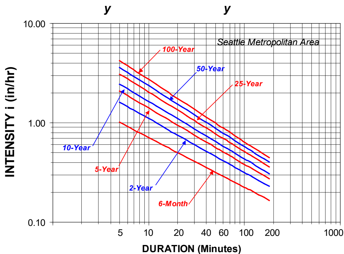
Figure F.18. Intensity-Duration-Frequency Curves for the City of Seattle.
