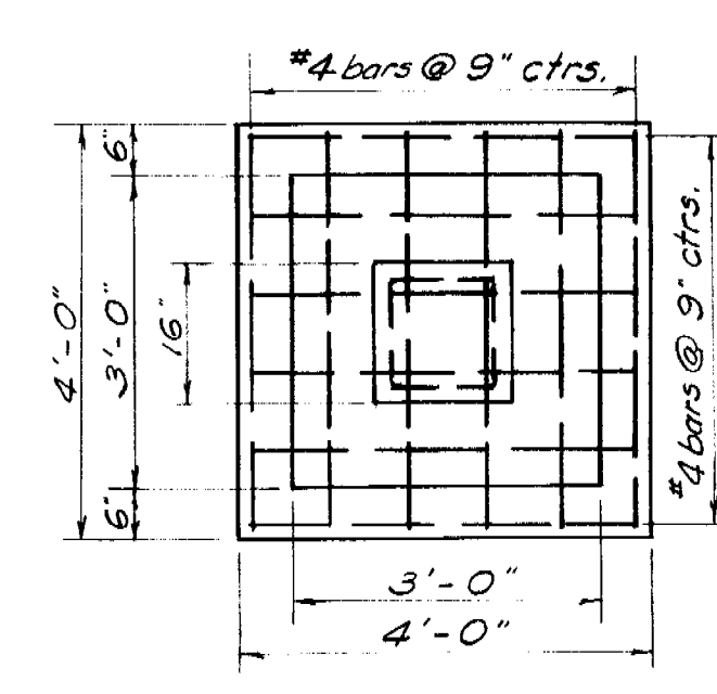
DETAIL E
