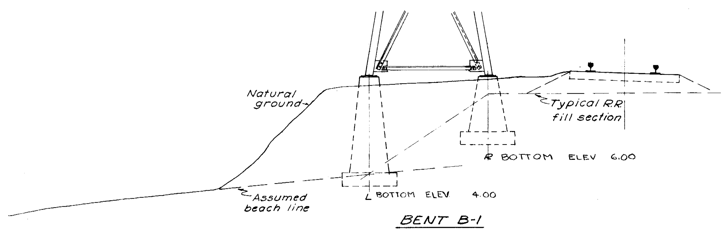
CROSS-SECTIONS
