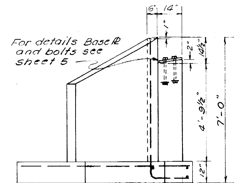
DETAIL A
