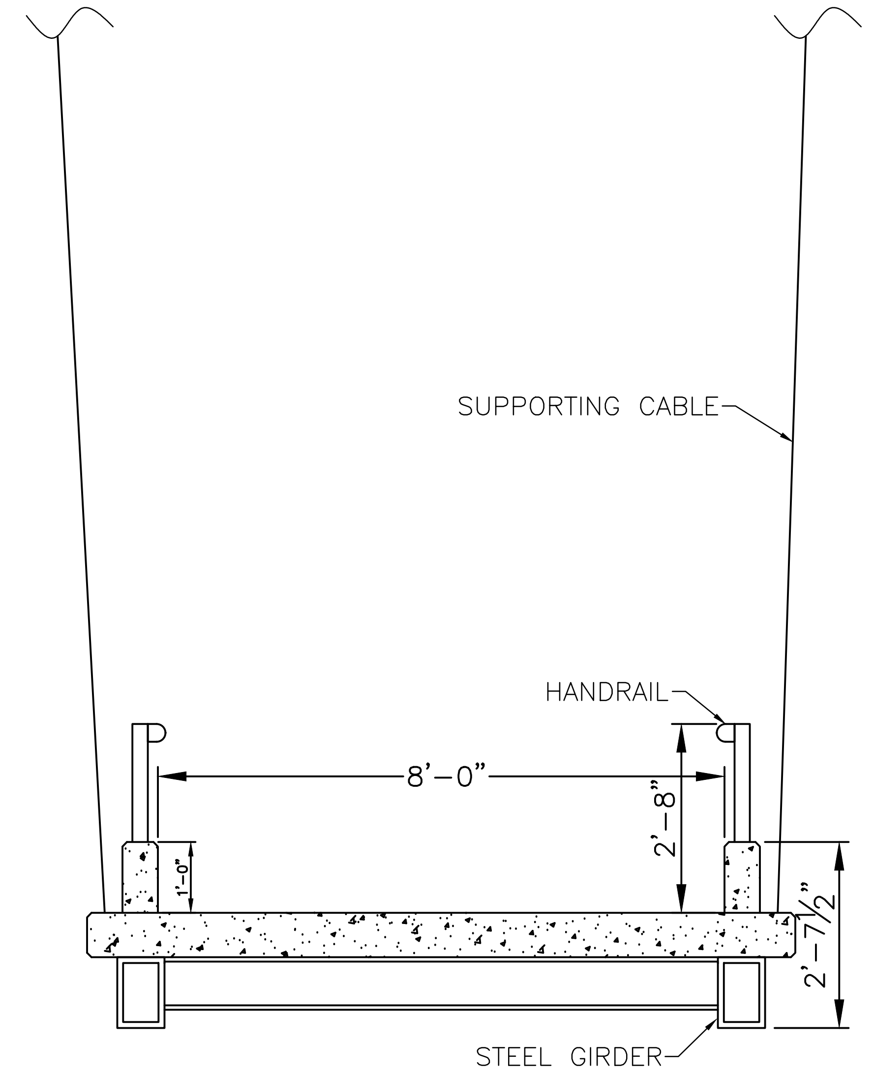
RAMP SECTION
