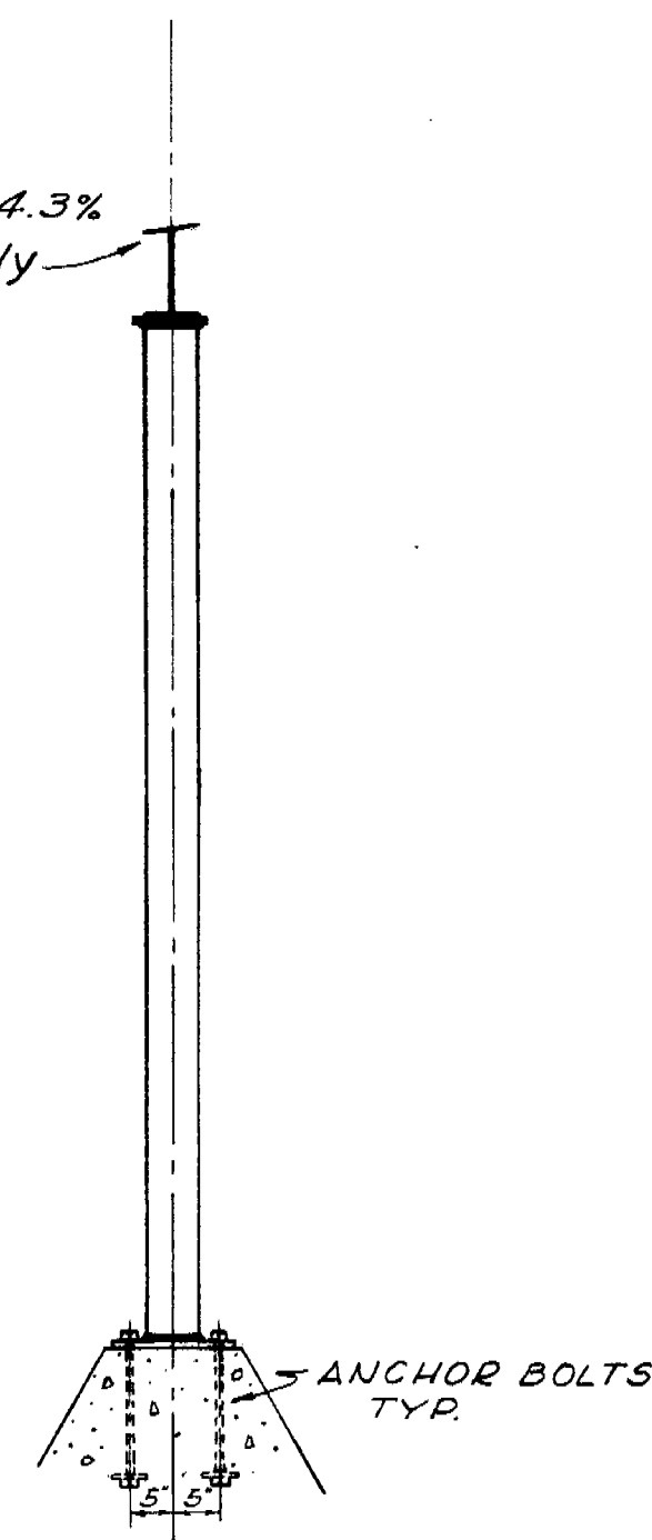
SECTION B-B
