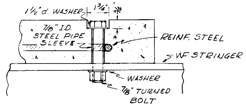
DETAIL H
