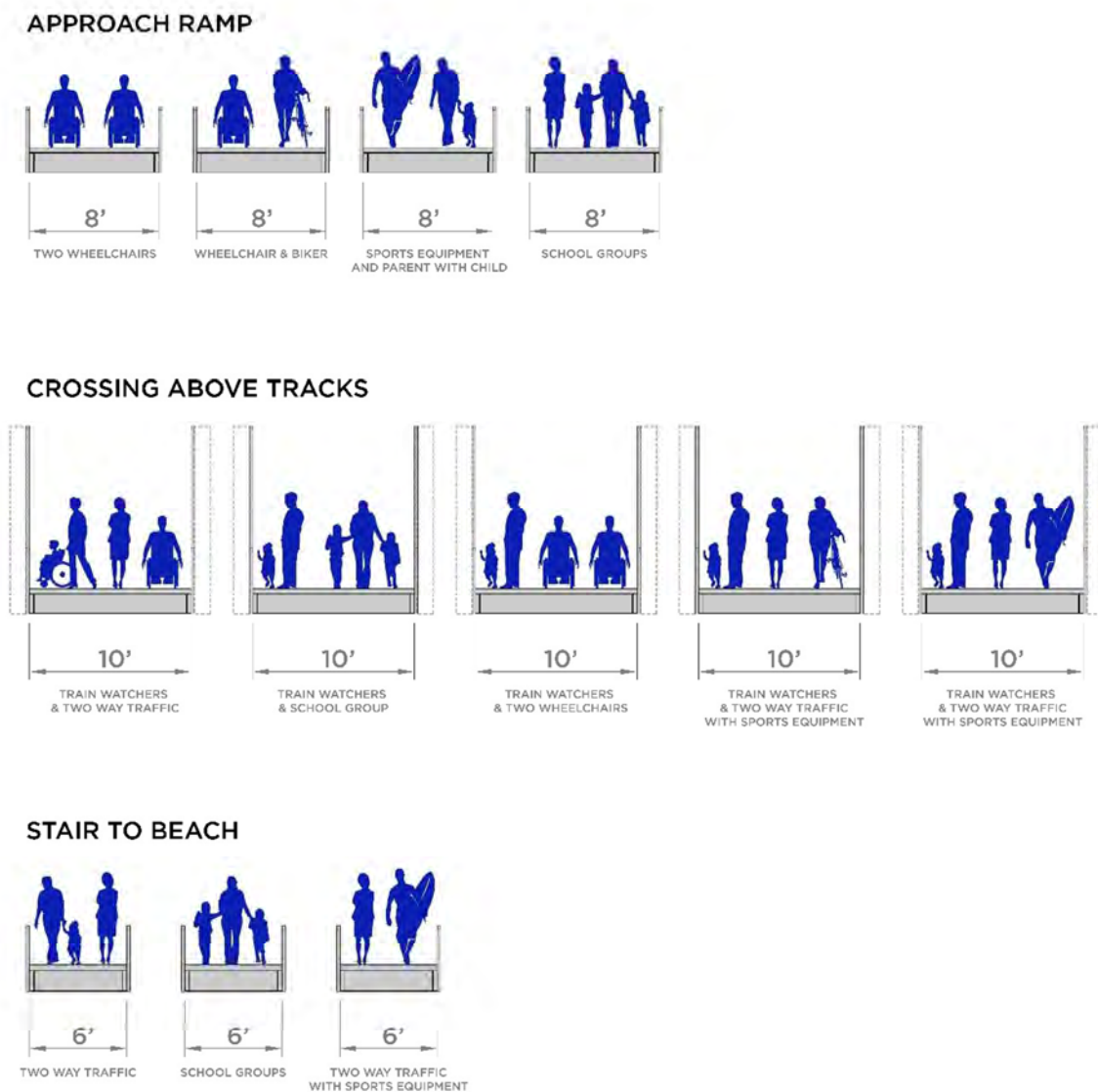
Figure 12 Bridge Sections
