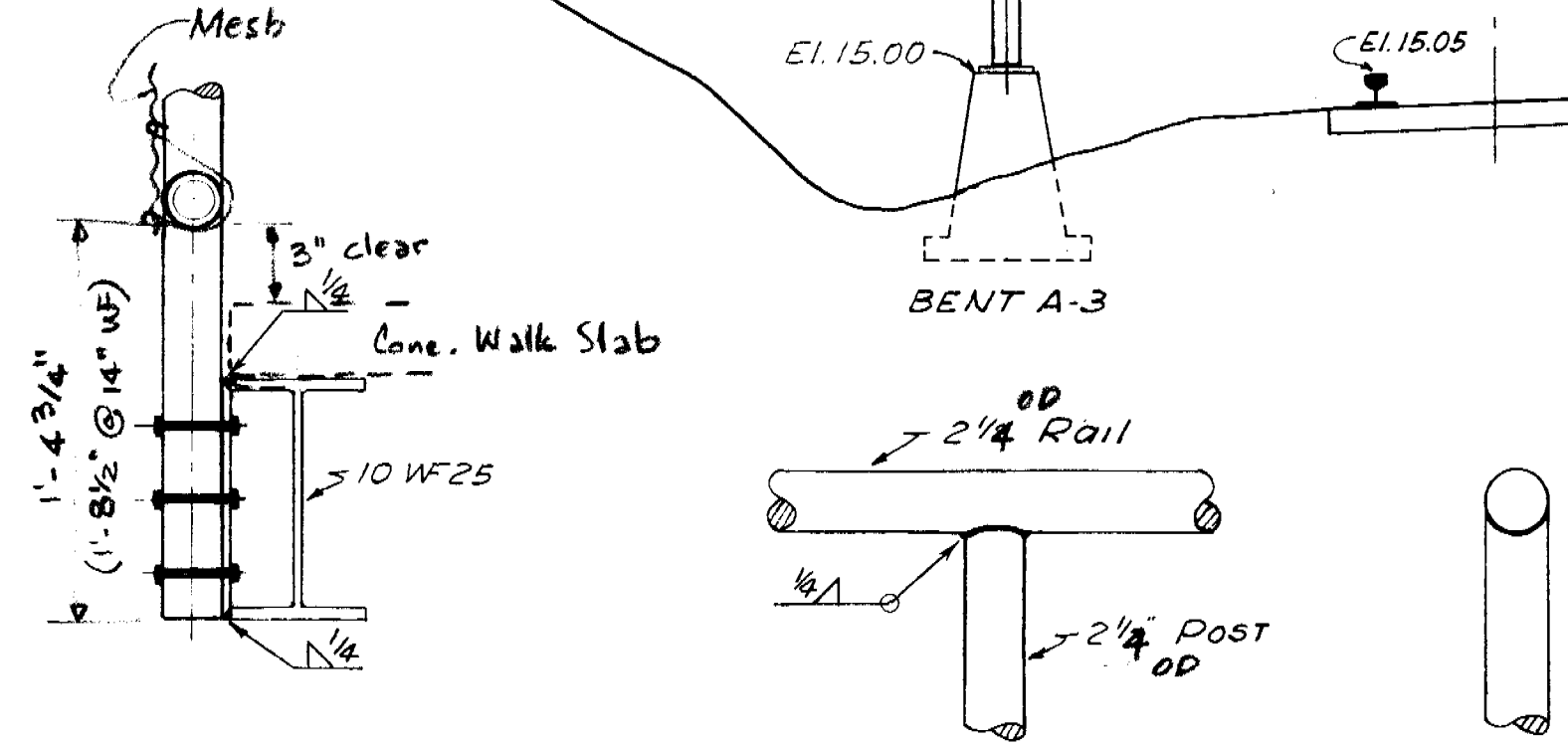
DETAIL D
