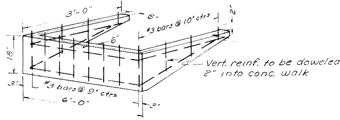
CUT-OFF WALL
