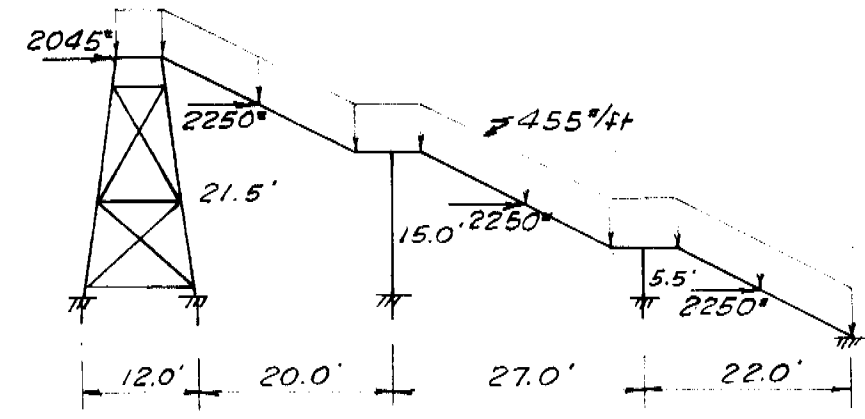
LOAD DIAGRAM
