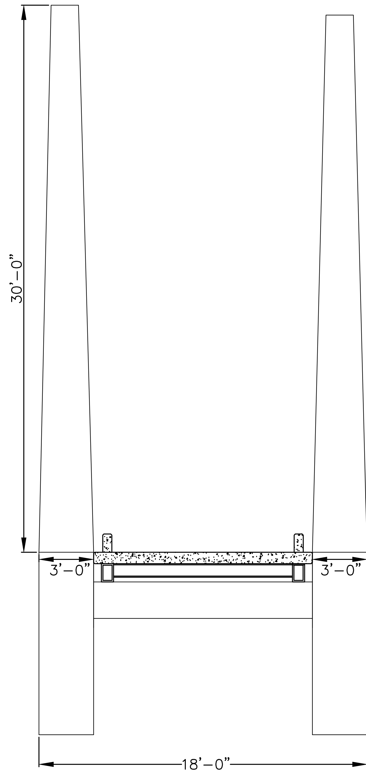
TOWER SECTION
