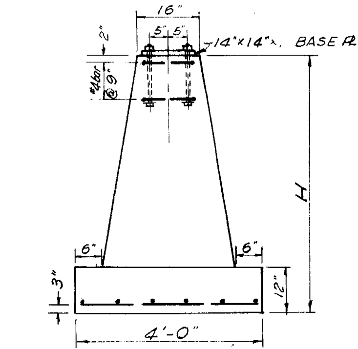
DETAIL E
