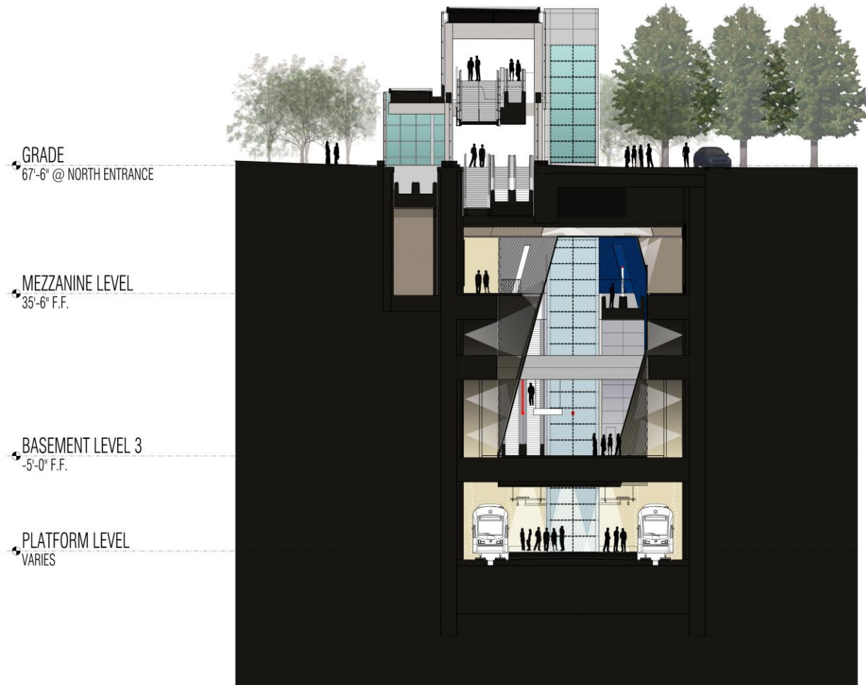
CROSS SECTION
