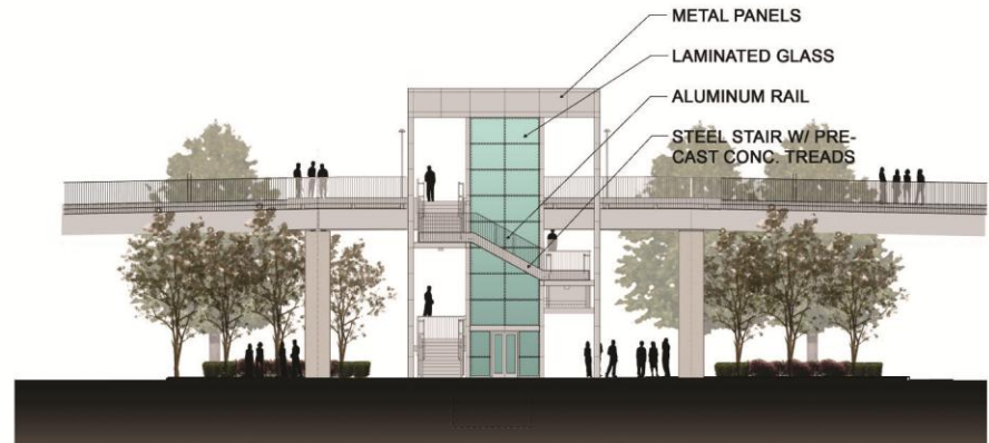
TRIANGLE STAIR - SOUTH ELEVATION
