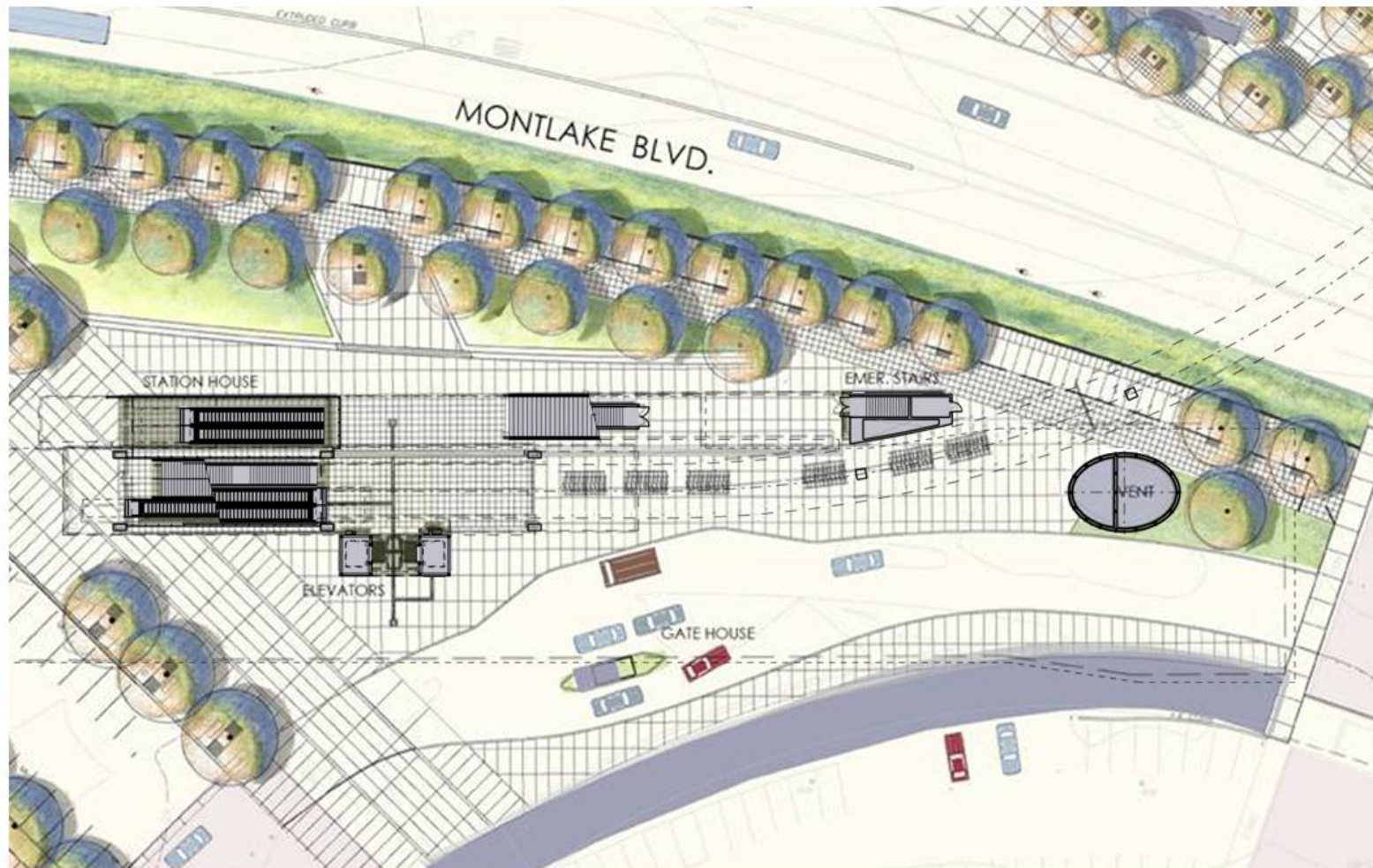
HEADHOUSE GRADE PLAN
