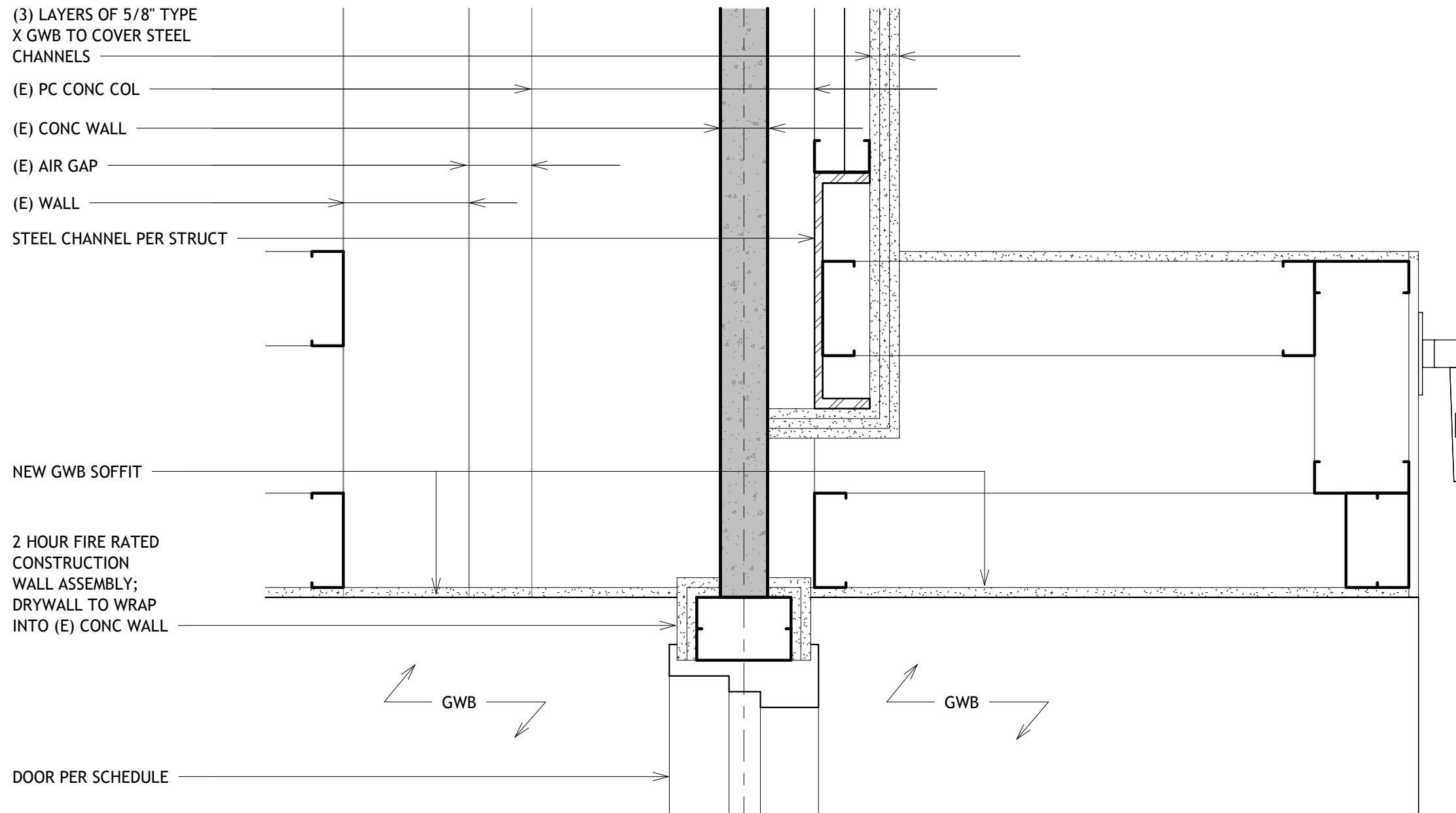
① EXHIBIT CIRCULATION - DOOR HEAD DETAIL 1 1/2" = 1'-0"
