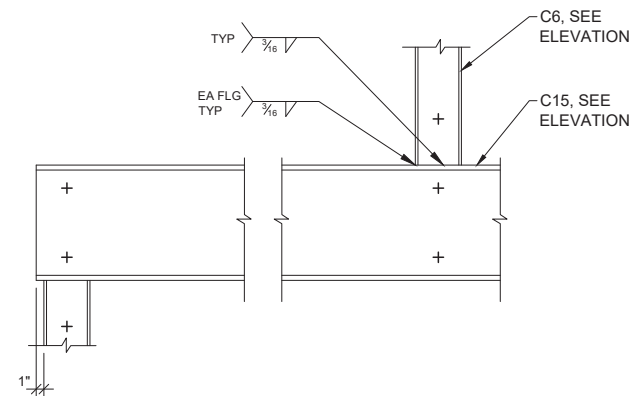
6 DETAIL 1/2"=1'-0"
