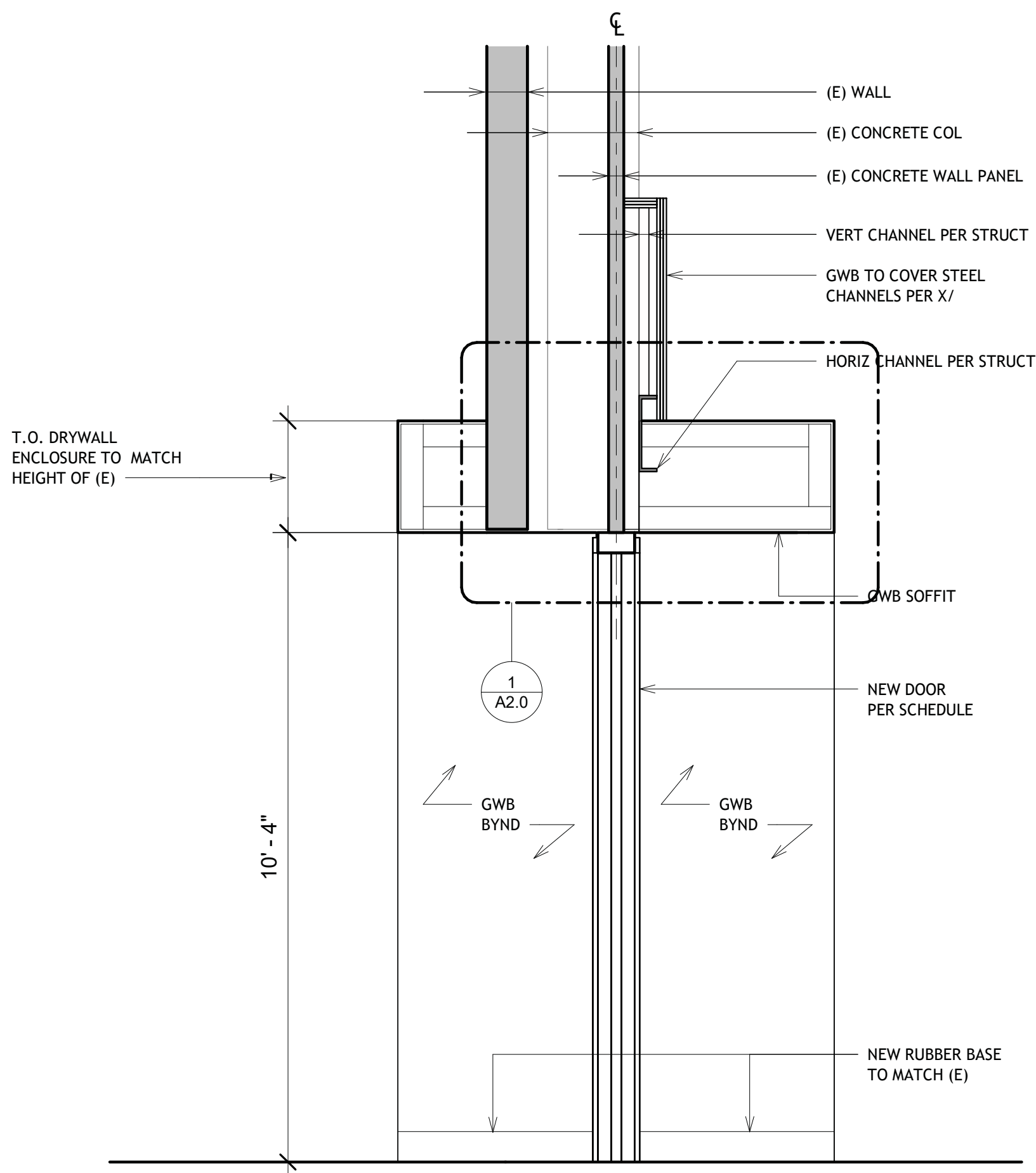
2 EXHIBIT CIRCULATION - DOOR SECTION 1/2" = 1'-0"
