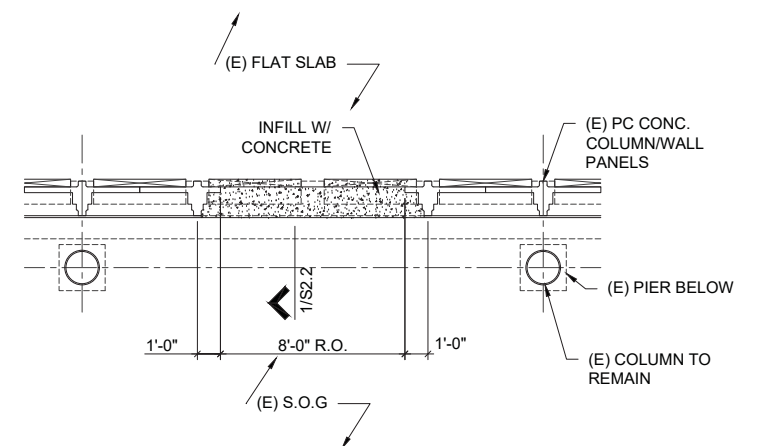
3 PARTIAL PLAN 1/8"=1'-0"
