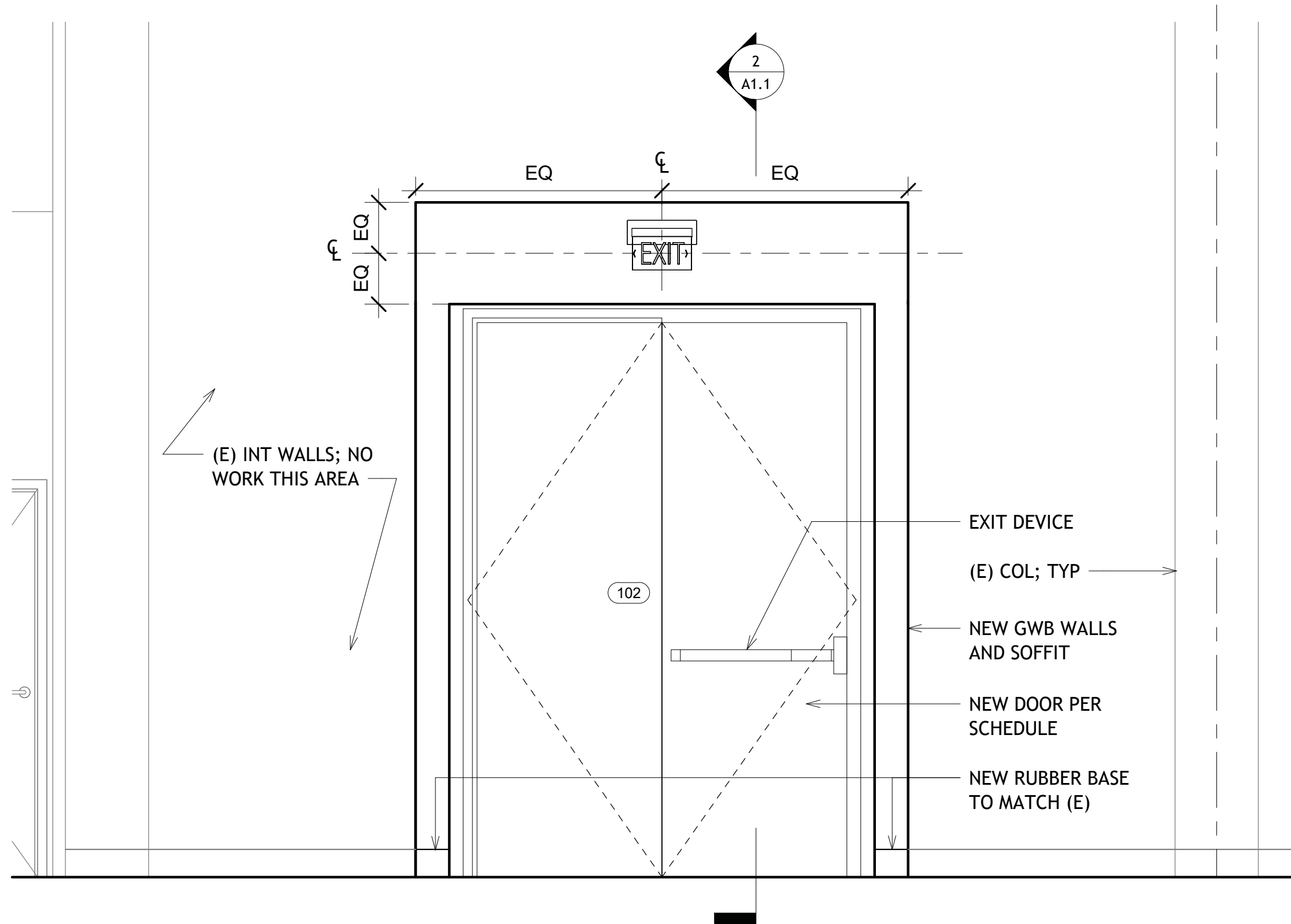
INT ELEVATION_DOOR_EXHIBIT CIRCULATION - WEST ③ 1/2" = 1'-0"
