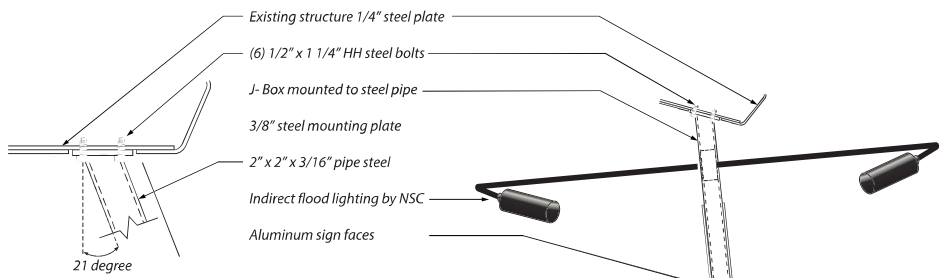
4 Section View- Enlarged Attachment Detail Scale: 1 1/2"=1'-0"
