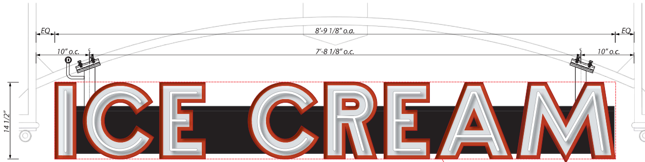
1 Front View Scale: 1"=1'-0"
