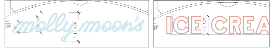
7 EAST SIGNAGE LETTER DIMENSIONS (PROPOSED)
