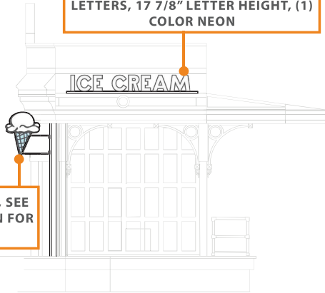
PROPOSED ELEVATION - NORTH SCALE: 1/8" = 1'-0"
