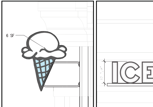
PROPOSED SIGNAGE DIMENSION - NORTH SCALE: 1/2" = 1'-0"
