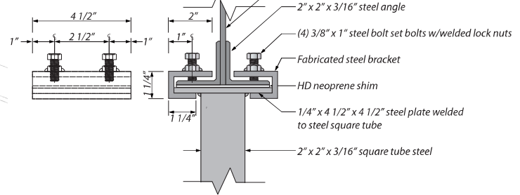
5 Side View- Enlarged Attachment Detail Scale: 3"=1'-0"
