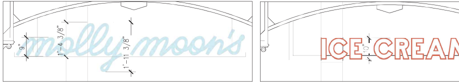
3 EAST SIGNAGE LETTER DIMENSIONS (ALLOWED)
