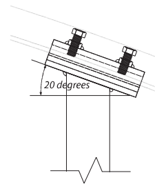
4 Enlarged Attachment Detail Scale: 3"=1'-0"
