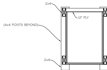
○ SECTION A
