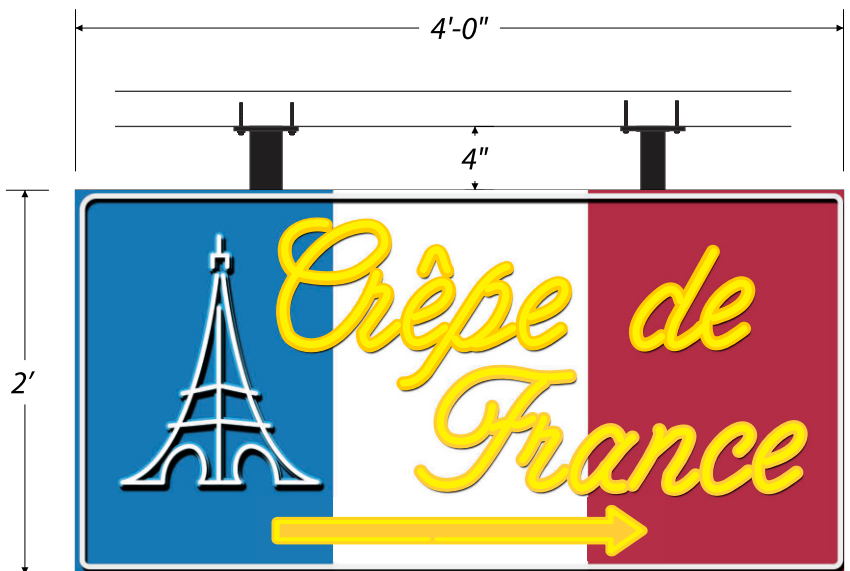
Side 2: Arrow to point to building both sides
