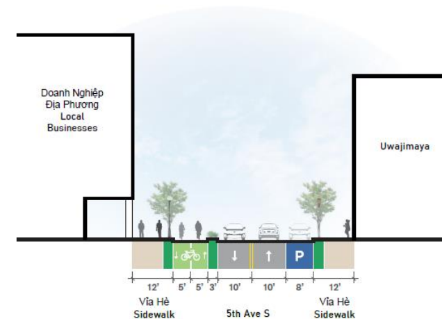
B Mặt cắt ngang 5th Ave S 5th Ave S cross section
