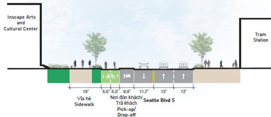
B Mặt cắt ngang Seattle Blvd S Seattle Blvd S cross section
