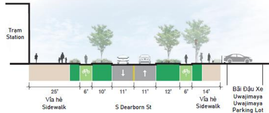
A Mặt cắt ngang S Dearborn St S Dearborn St cross section
