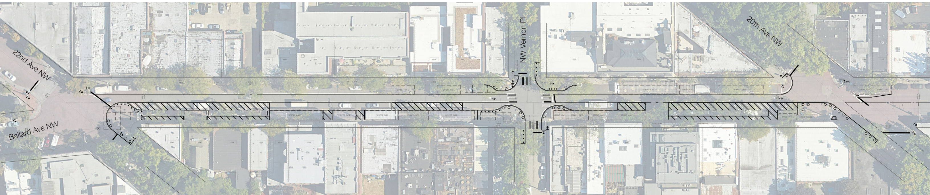
Existing striping and planters between 20th Ave NW and 22nd Ave NW
