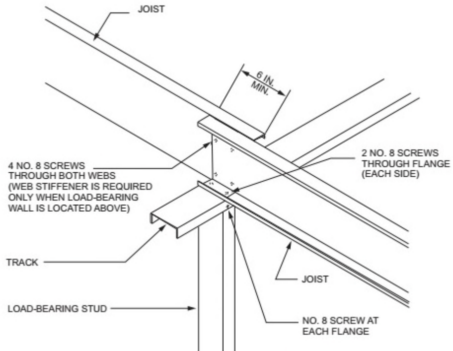
FIGURE R505.3.1(8) LAPPED JOISTS SUPPORTED ON INTERIOR LOAD-BEARING WALL
