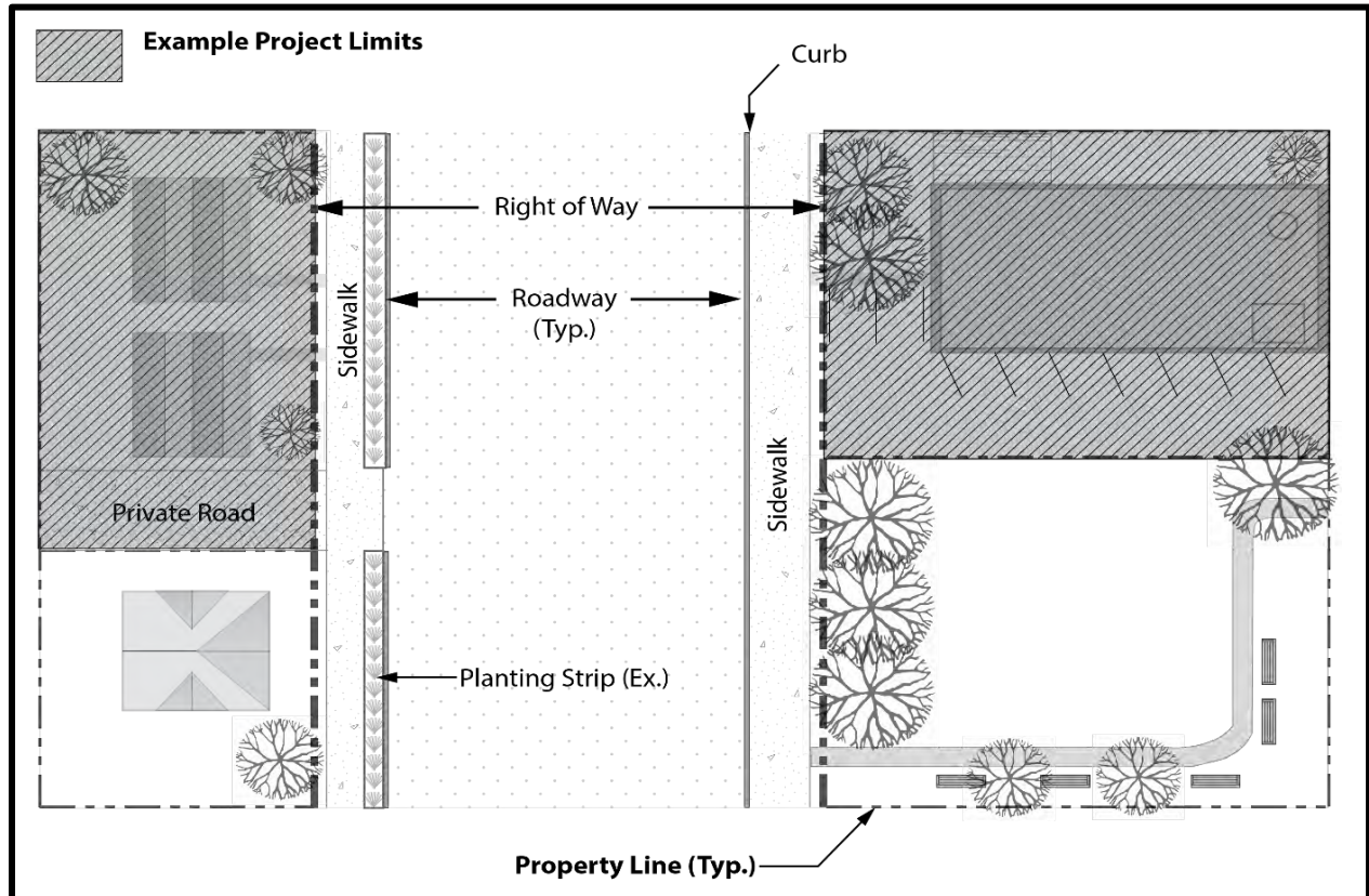
Figure 2.5. Parcel-Based Project Site Definition.
