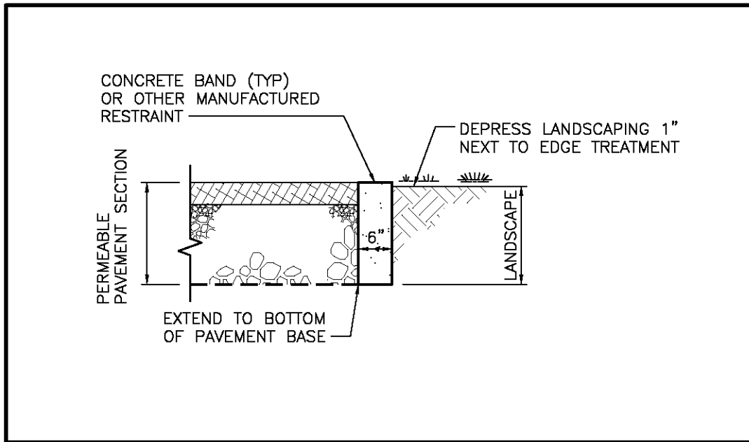
Figure 5.19. Example Permeable Pavement Concrete Edge Treatment.
