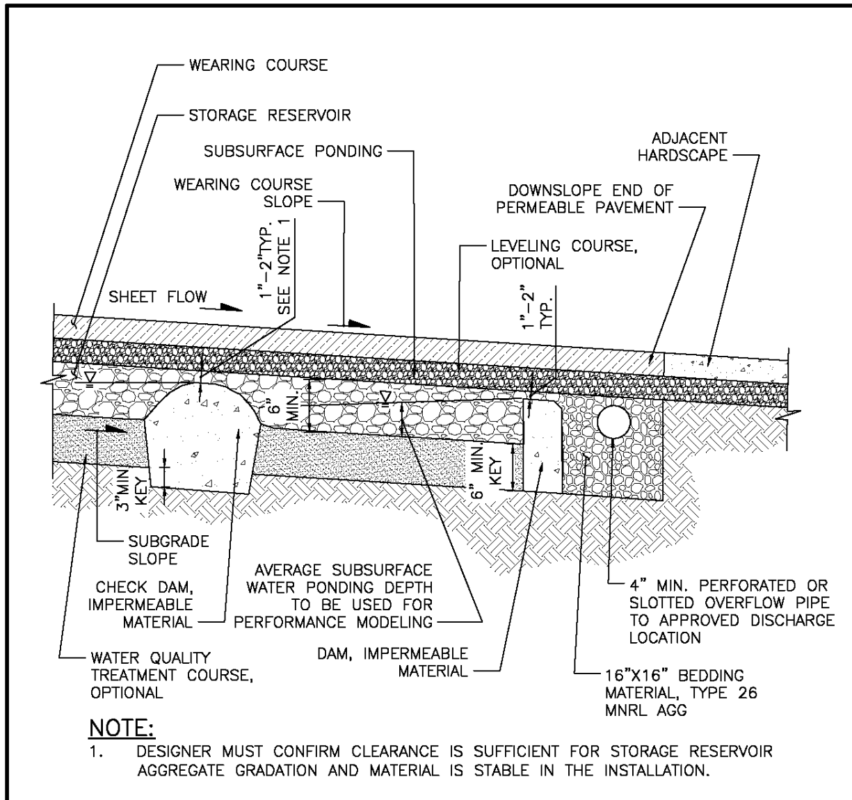
Figure 5.185-16. Typical-Example Permeable Pavement Facility with Checkdams.
