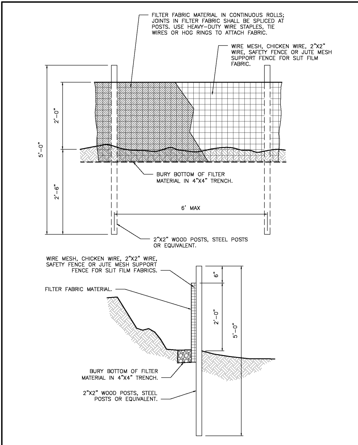
Figure 14. Silt-Filter Fence Details.
