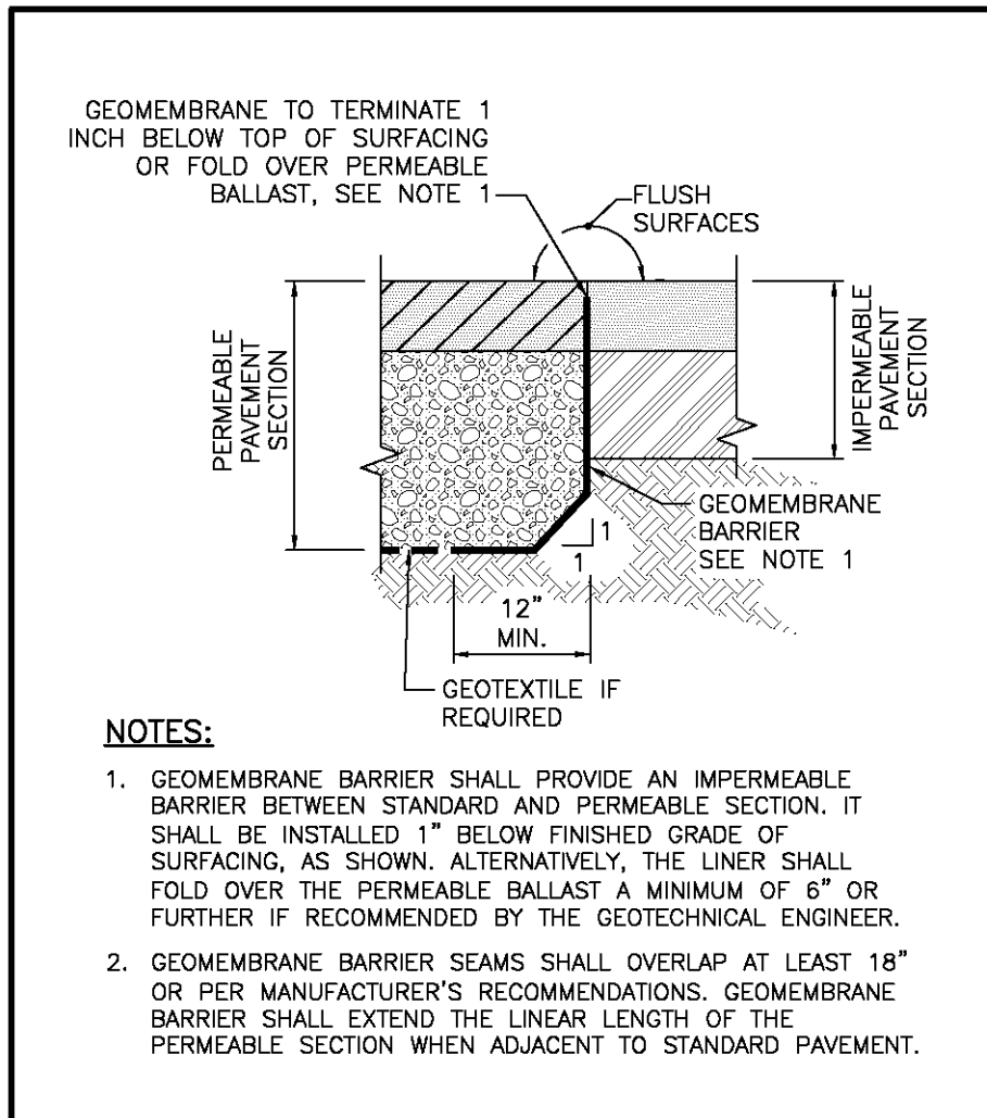
Figure 5.20. Example Permeable Pavement Geomembrane Edge Treatment.
